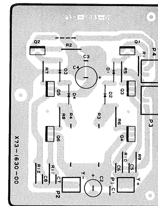
V. FINAL AMP UNIT (X73-1630-00)
