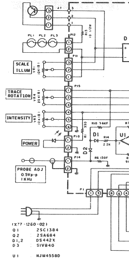
CONNECTION UNIT (X77-1260-02)
