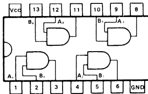
SN74LS08N
