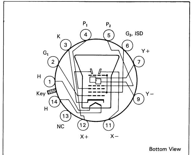
Fig. 2 150GTM31A Basing
